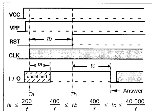
Figure 2 — Activation and cold reset
