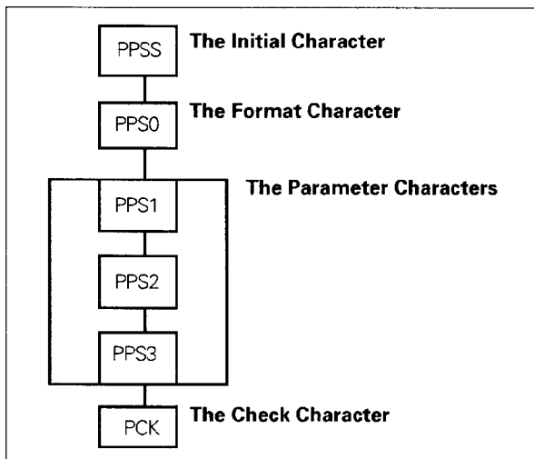
Figure 15 — Structure of PPS request and response
