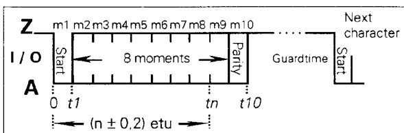
Figure 7 — Character frame
