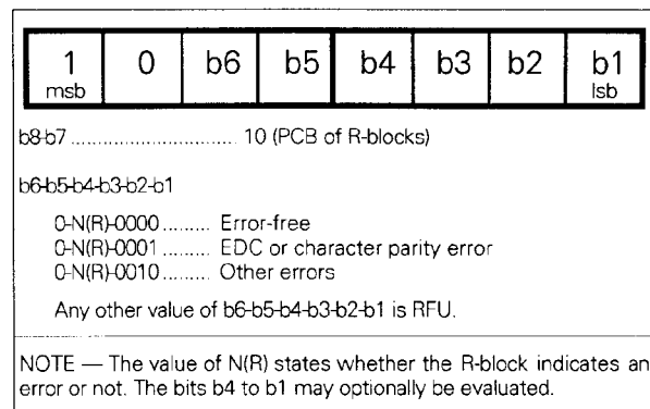
Figure 18 — Coding of R-block PCB
