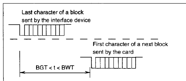
Figure 21 — Block waiting time and block guardtime
