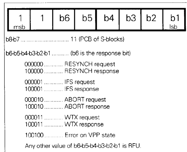
Figure 19 — Coding of S-block PCB
