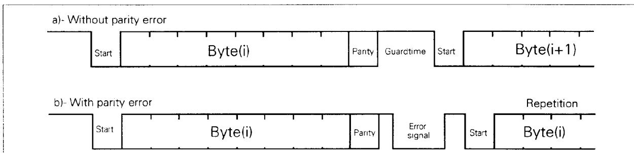
Figure 8 — Character transmission and repetition diagram
