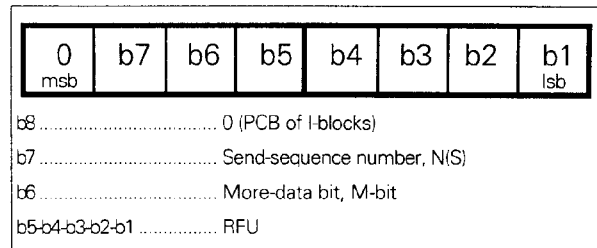
Figure 17 — Coding of I-block PCB
