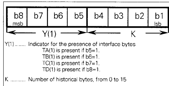
Figure 11 — Coding of T0
