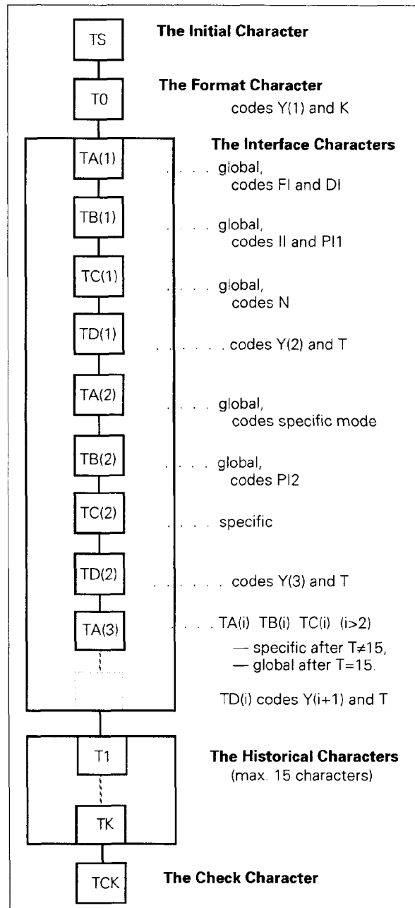
Figure 6 — Configuration of the Answer-to-Reset
