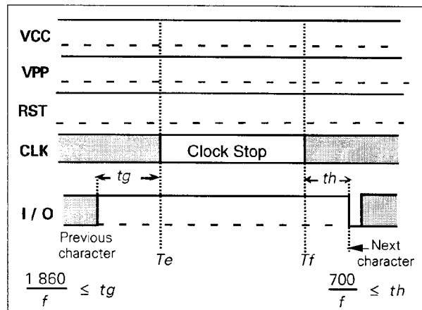
Figure 4 — Clock stop
