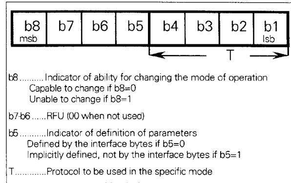
Figure 13 — Coding of TA(2)
