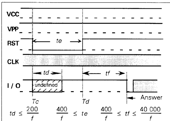
Figure 3 — Warm reset
