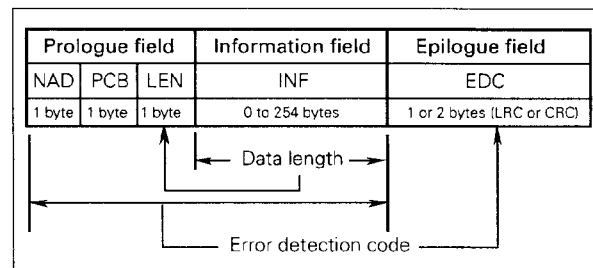
Figure 16 — Block frame
