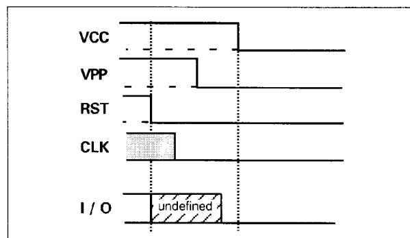
Figure 5 — Deactivation
