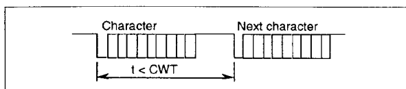
Figure 20 — Character waiting time
