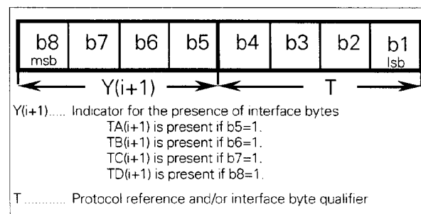
Figure 12 — Coding of TD(i)
