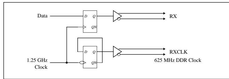
Figure 5 Reference data and clock circuit
