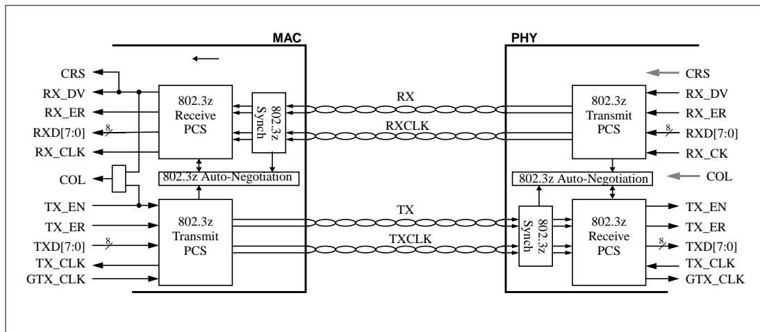
Figure 1 SGMII Connectivity
