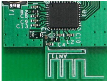
Figure 5. PCB 天线
