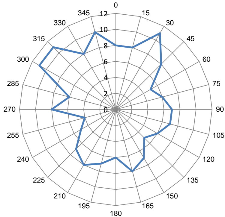
Figure 9.辐射图
